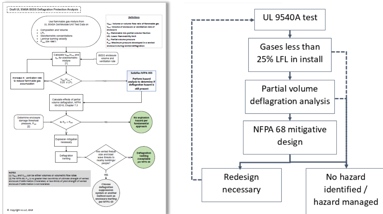
Figure 3 Deflagration Protection Analysis (left: full chart, right: simplified chart)
