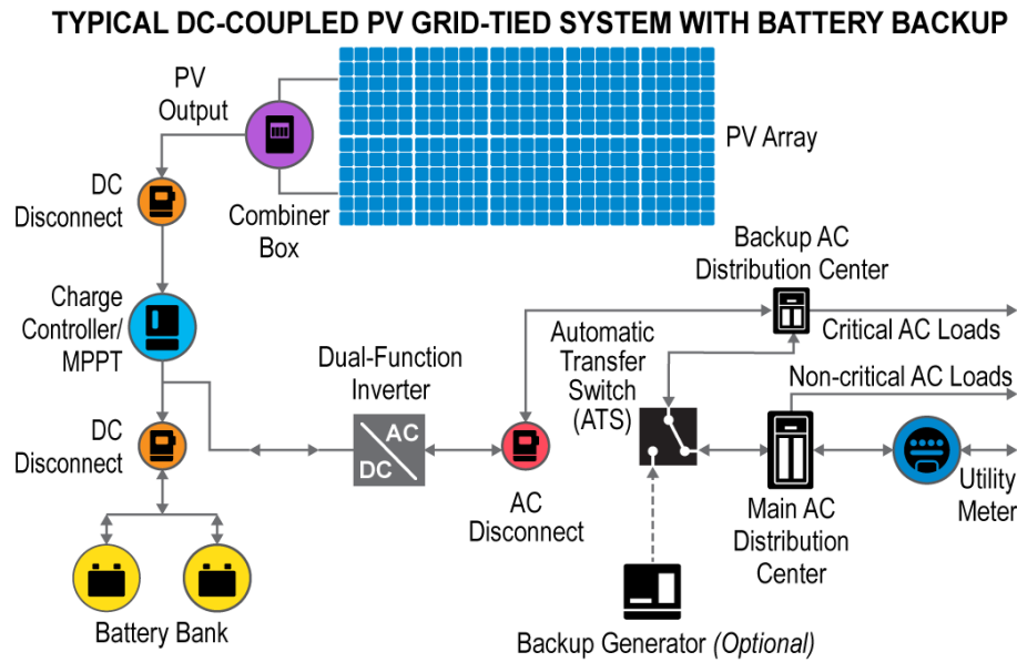
Figure 2: DC-Coupled Resilient PV
