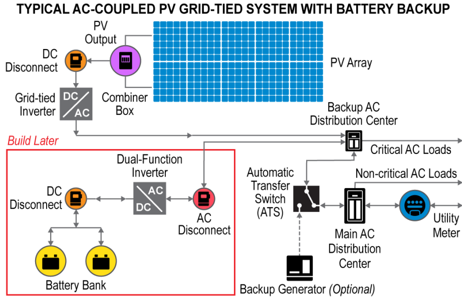
Figure 5: AC- Coupled Storage Ready Schematic
