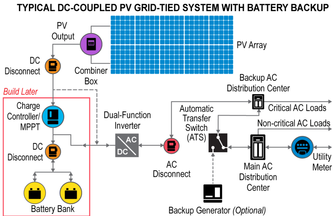
Figure 4: DC-Coupled Storage Ready Schematic
